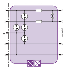
Basic circuit diagram BXT ML2 BD S EX 24
